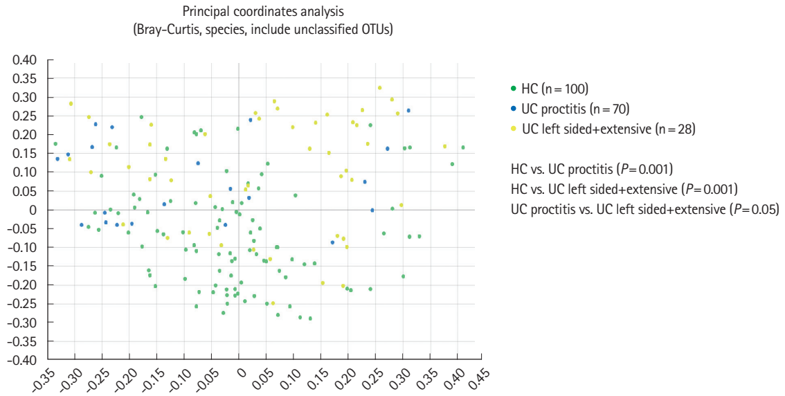
Supplementary Fig. 1. Beta diversity based on Bray-Curtis index according to the disease extent in patients with ulcerative colitis (UC). HC, healthy control individuals; CD, Crohn's disease; OUT, operational taxonomic unit.
